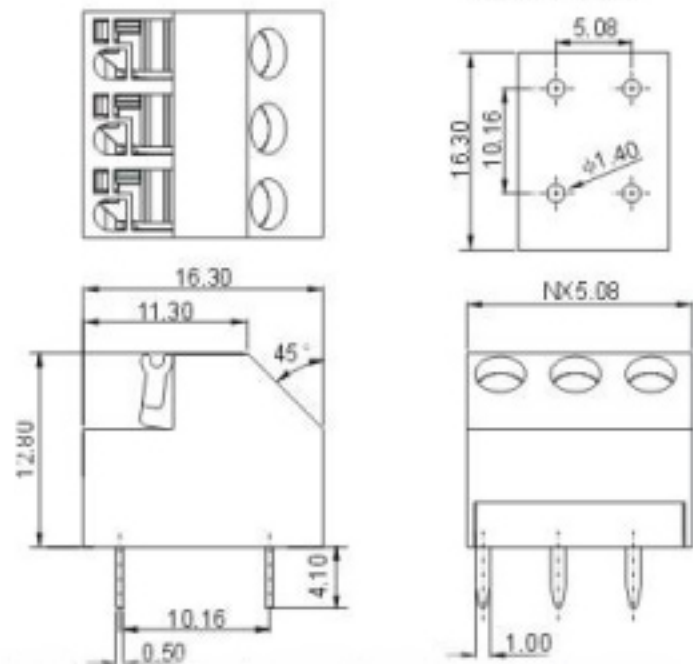
PCB LAYOUT
