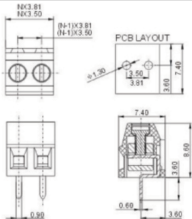
KV381-3.5/3.81
